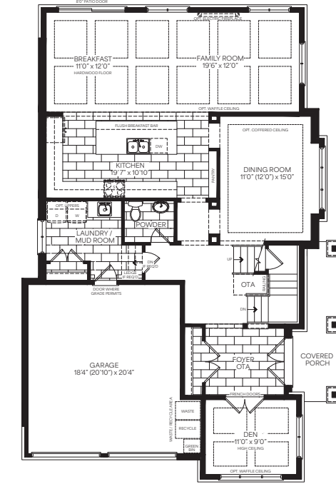
Main Floor Elevation B
