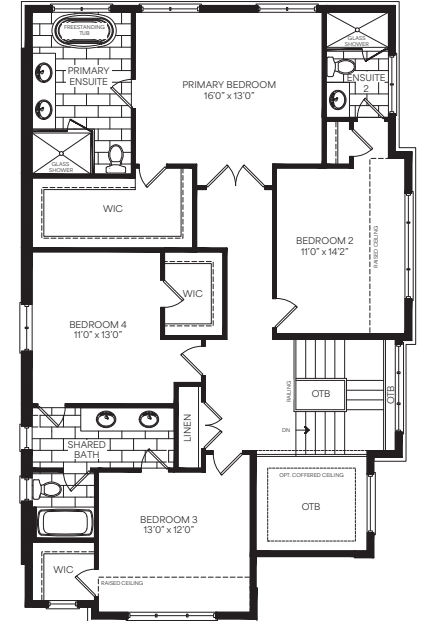
Second Floor Elevation C
