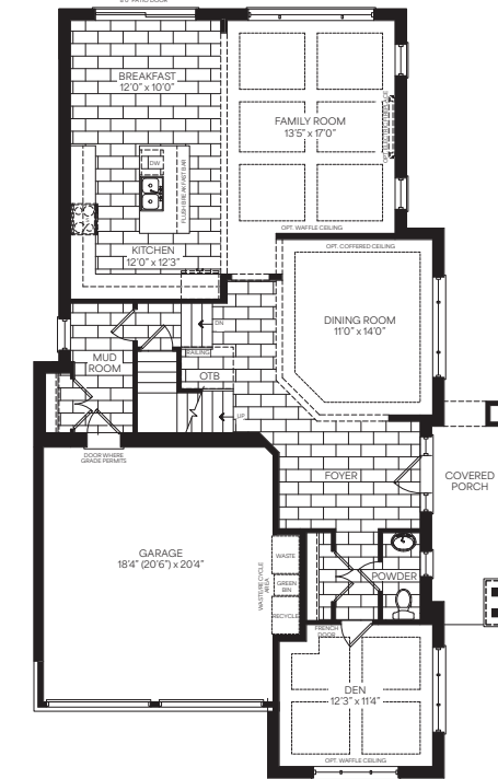
Main Floor Elevation C
