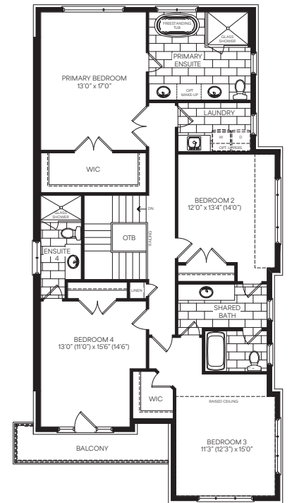
Second Floor Elevation C
