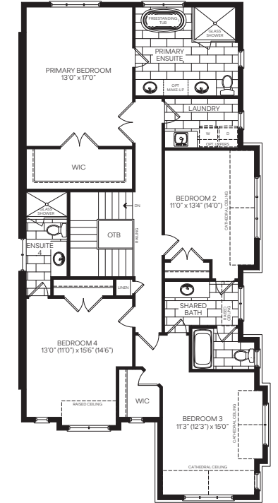
Second Floor Elevation B
