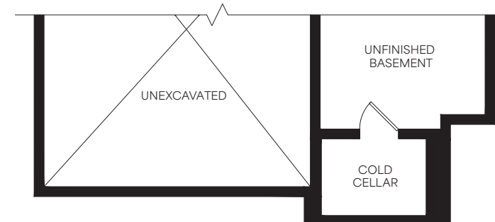
Basement Elevation C
